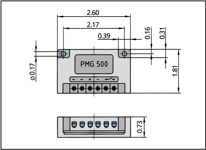
Figure 4.1: PMG 500 Dimensions
