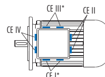
Conduit Entry Positions (Position M1 shown)
